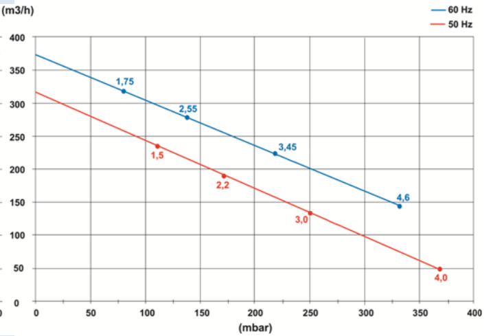
Ansaugvolumenstrom / Suction air flow
