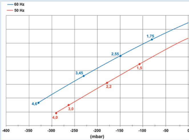
Ansaugvolumenstrom / Suction air flow
