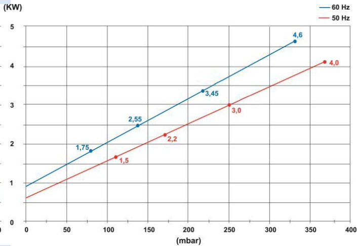
Wellenleistung / Power requirement on the blower shaft
