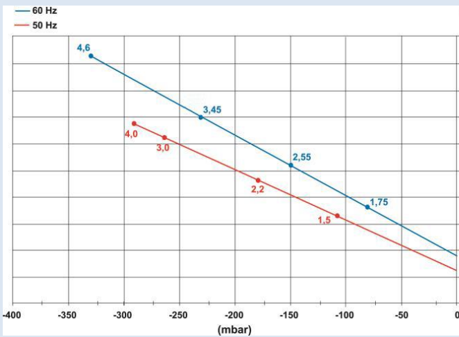
Wellenleistung / Power requirement on the blower shaft
